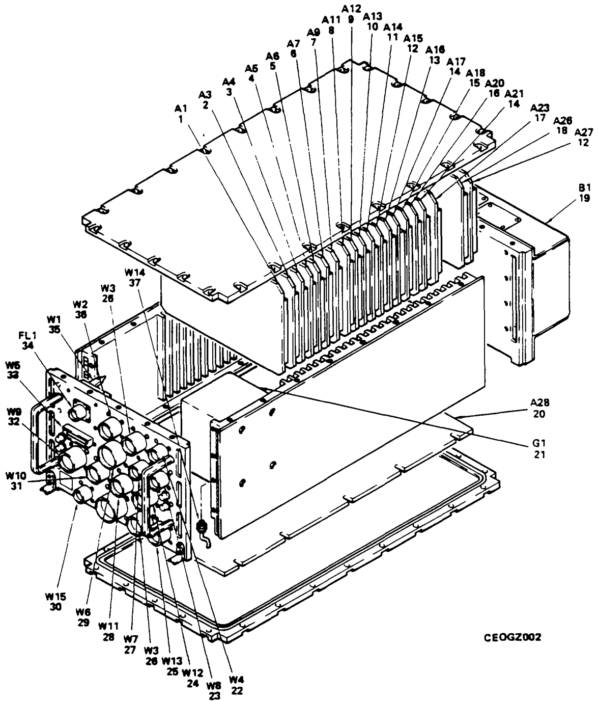
Figure 1. Interface Unit J-4522/U (Sheet 1 of 4)
